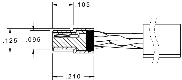
SECTION A-A VIEW LESS HARDWARE AND SHRINK TUBES
